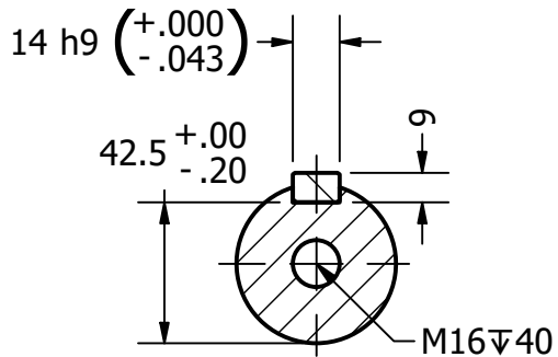
SECTION A-A SCALE 2:5
