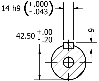
SECTION A-A SCALE 2:5
