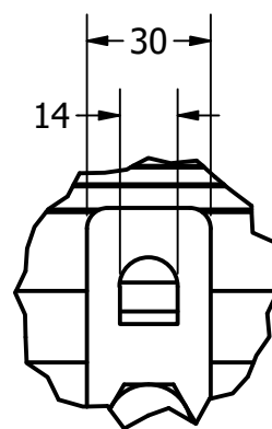
DETAIL B SCALE 1:2
