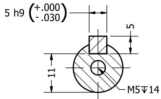
SECTION A-A SCALE 3:2
